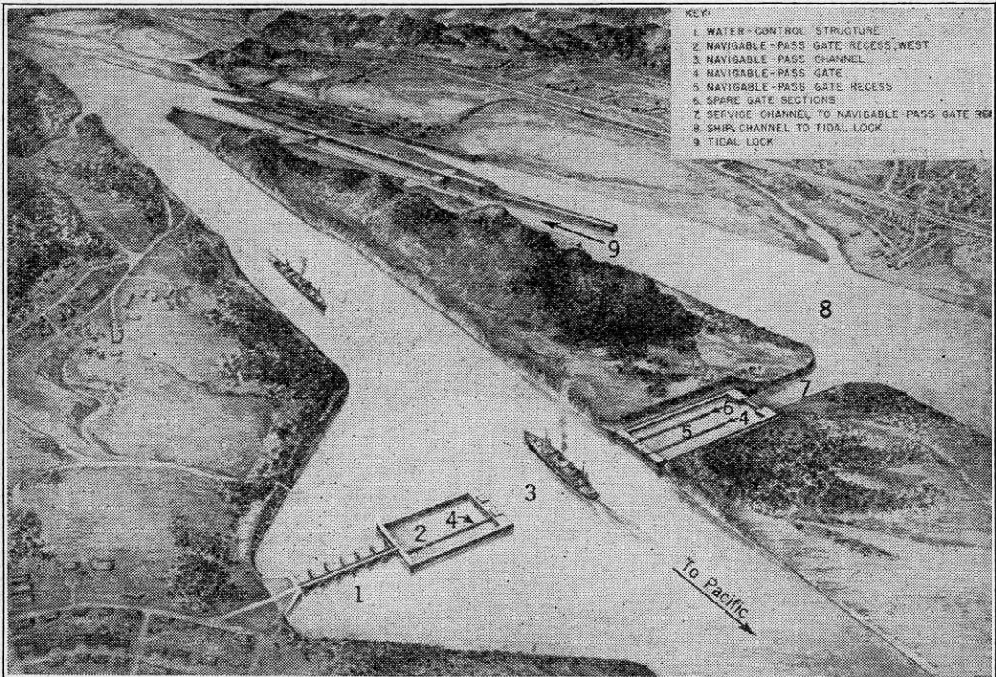
FIG. 37.—LAYOUT OF TIDAL-REGULATING STRUCTURES
